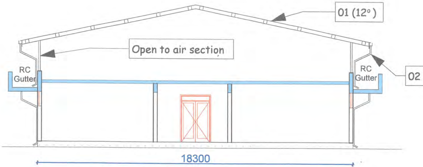
SECTION THROUGH THEATRE (27m Long)
