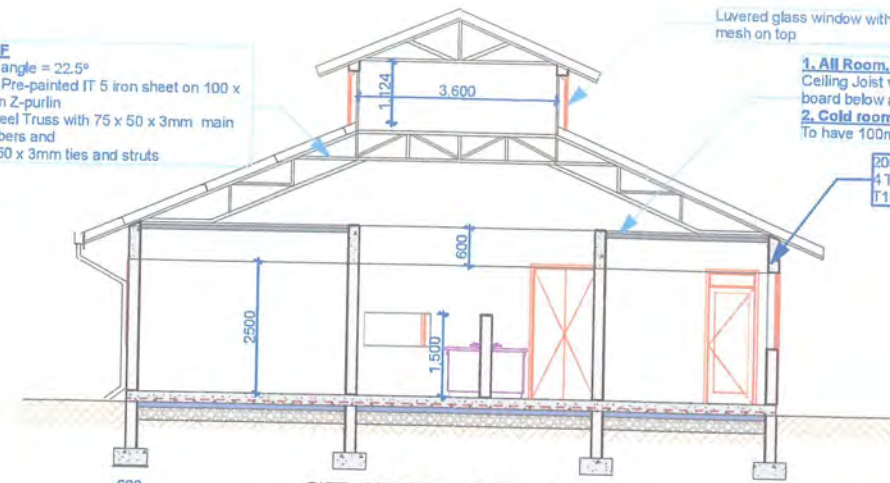
SECTION X-X
