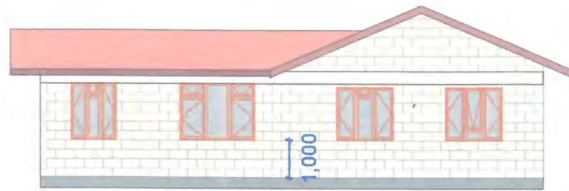
REAR ELEVATION
