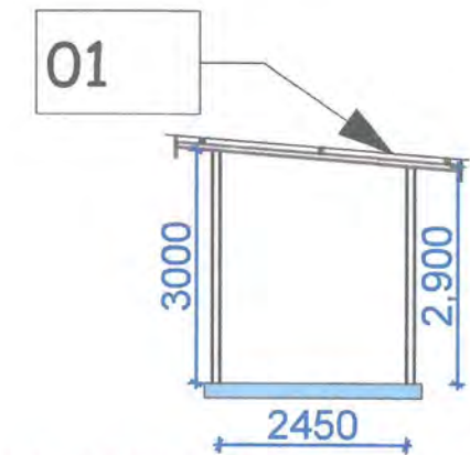
SECTION THROUGH WALK-WAY (207 m Long)
