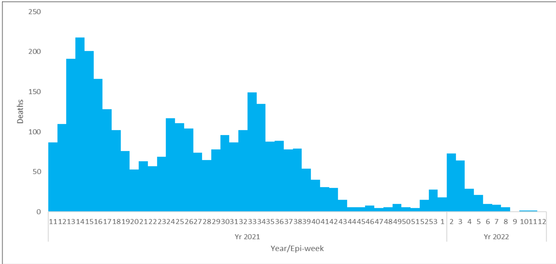
Figure 2: Trends of COVID-19 deaths in Kenya in the last one year
